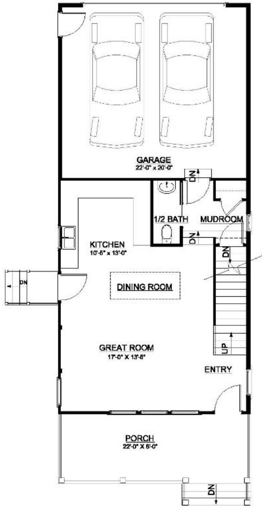
MAIN FLOOR - 610 SF
